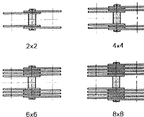
Plate lacing
